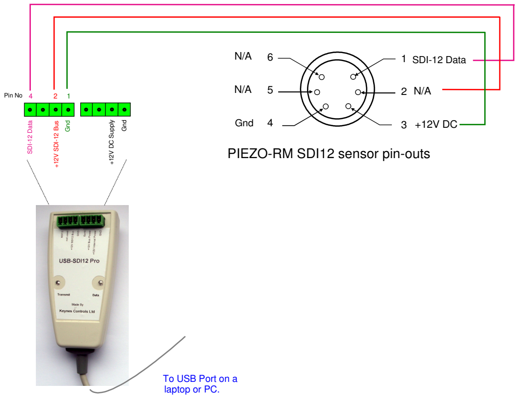
Part No. USB-SDI12-Pro
